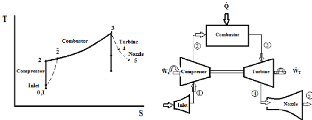
Figure (1) Brayton Cycle for Jet propulsion [7]
